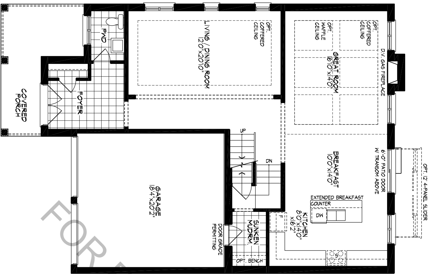
GROUND FLOOR PLAN, EL. 'A'
