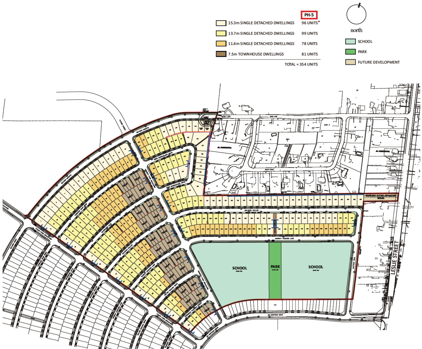
Phase 5 Master Plan not to scale (final layout subject to change)
